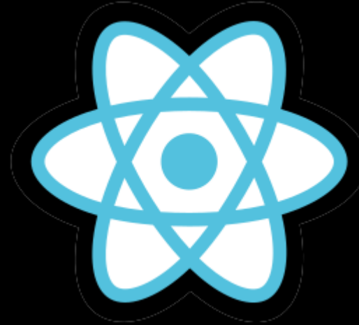
ReactJS
